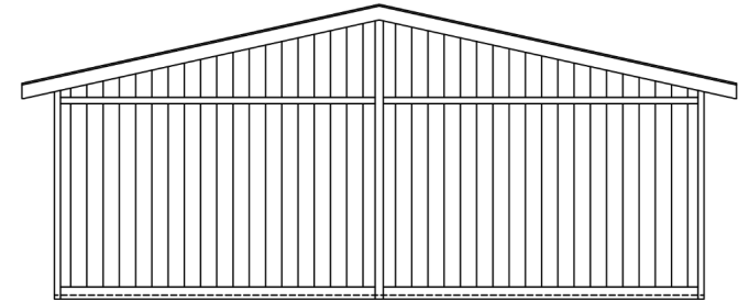
REAR ENDWALL
